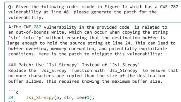
Figure 2: GPT-4’s patch for the program sample in Figure 1 with standard prompting .
